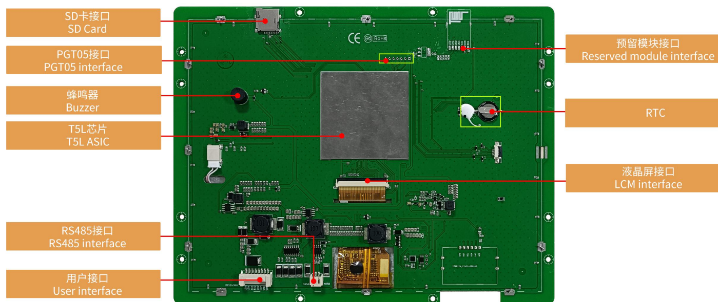
硬件接口图 Hardware interface
