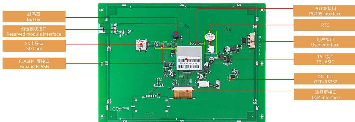
硬件接口图 Hardware interface
