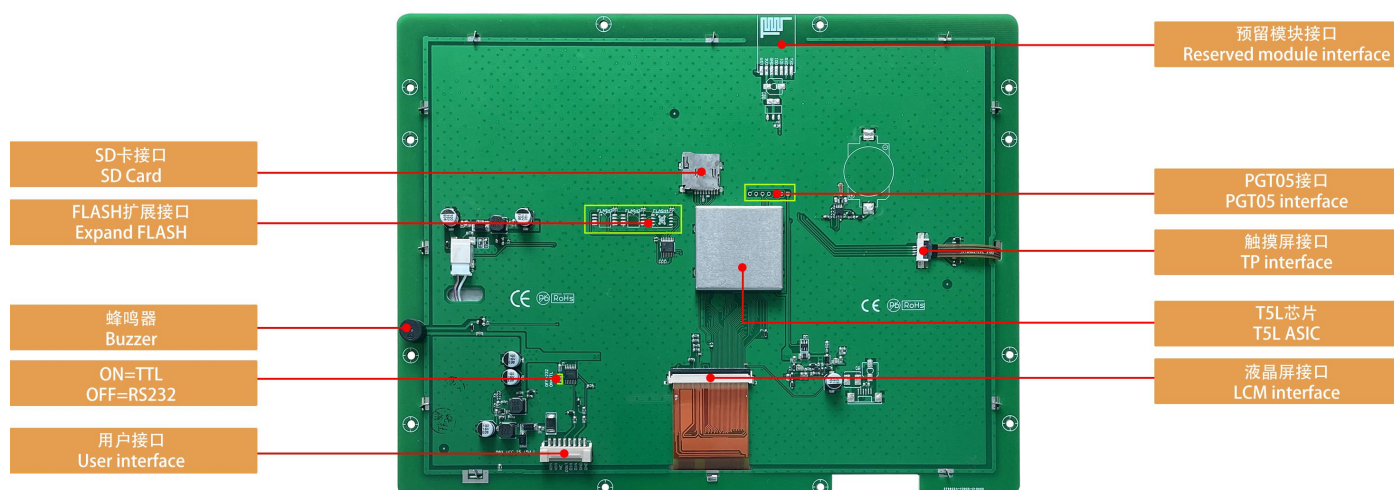
硬件接口图 Hardware interface
